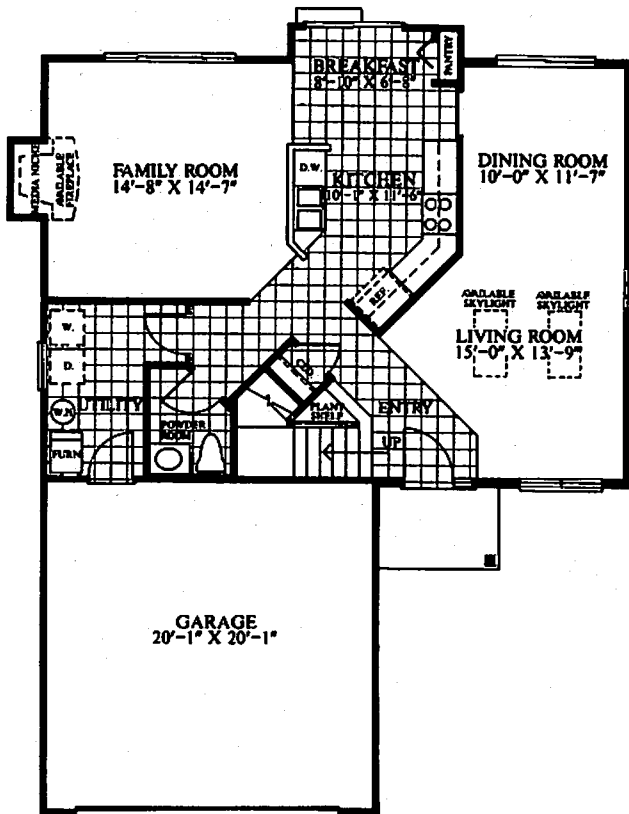
FIRST FLOOR PLAN WINDOW LOCATIONS VARY PER ELEVATION
