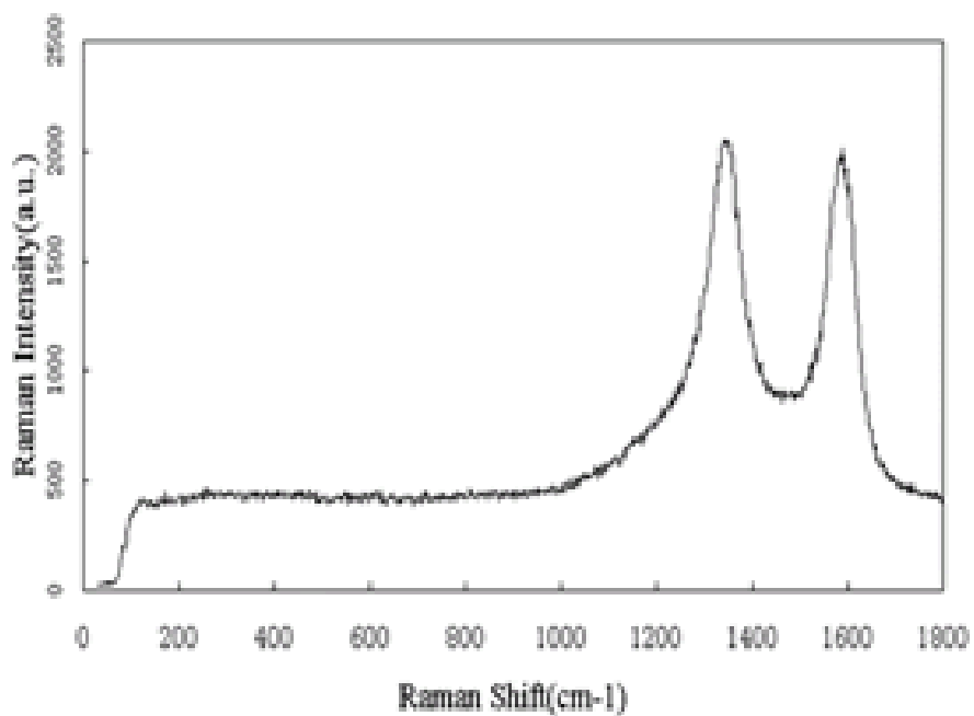
Raman Spectrum of MWCNTs With OD 8-15nm
