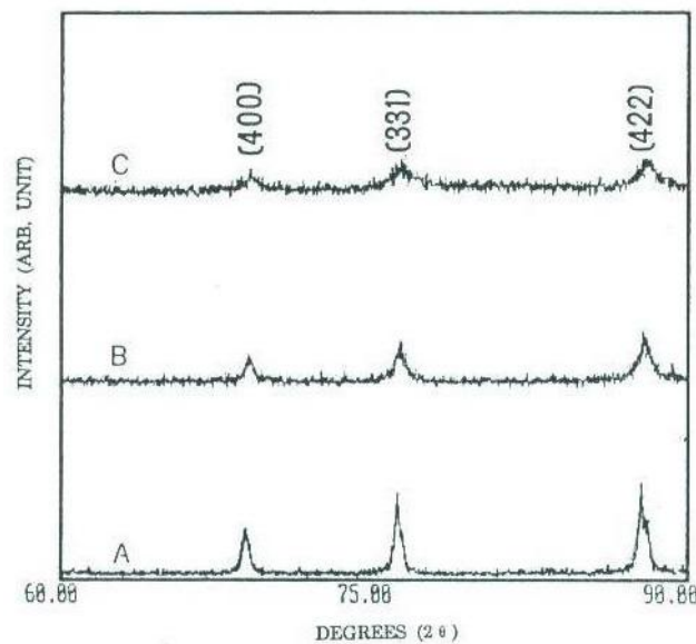
Si nanopowder X-ray (A:50-70nm;B:30-50nm;C:20-30nm)
