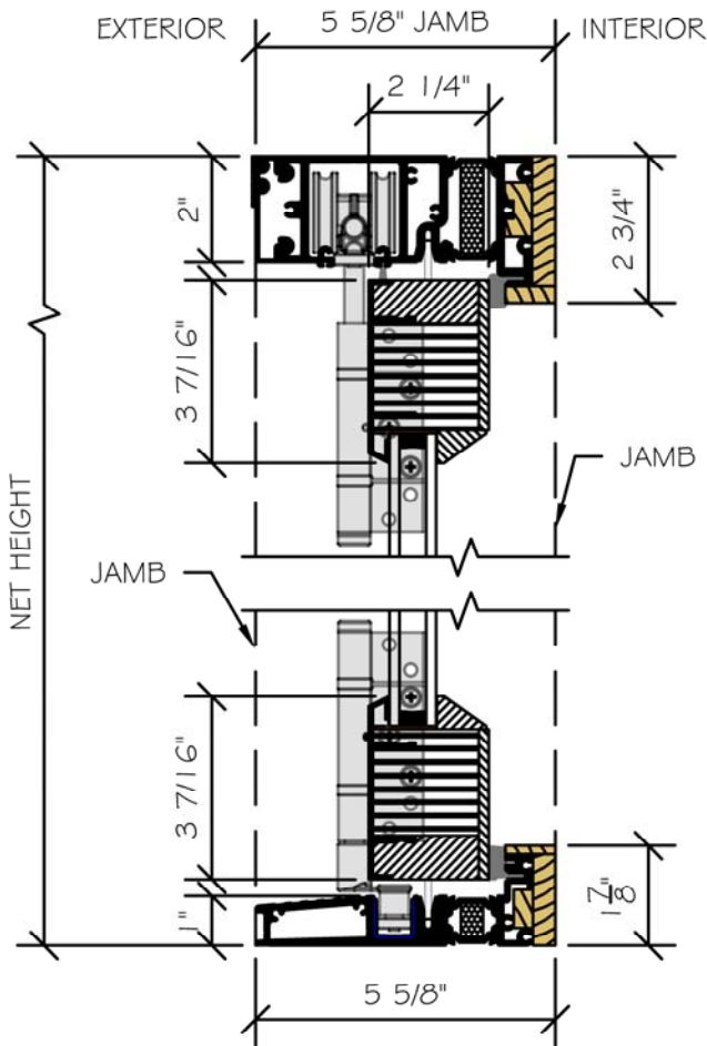
SECTION VIEW
