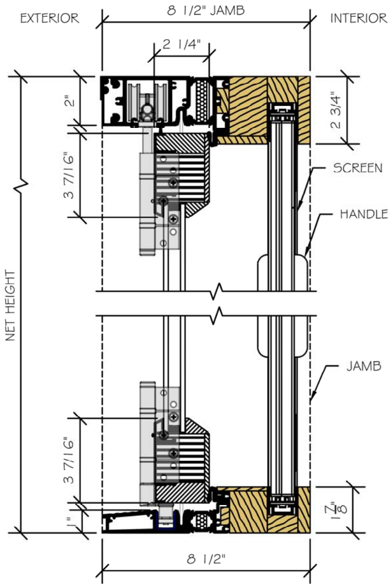
SECTION VIEW
