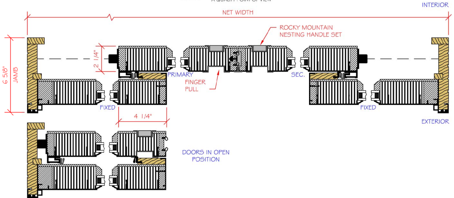
PLAN VIEW LIFT & SLIDE (OX XO) (TRADITIONAL CLAD) W/ROCKY MOUNTAIN NESTING HANDLE SET (UPCHARGE APPLIES) SCALE: 3" = 1'-0
