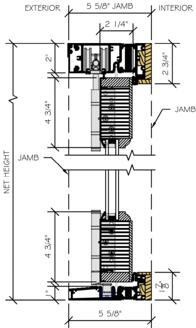
SECTION VIEW
