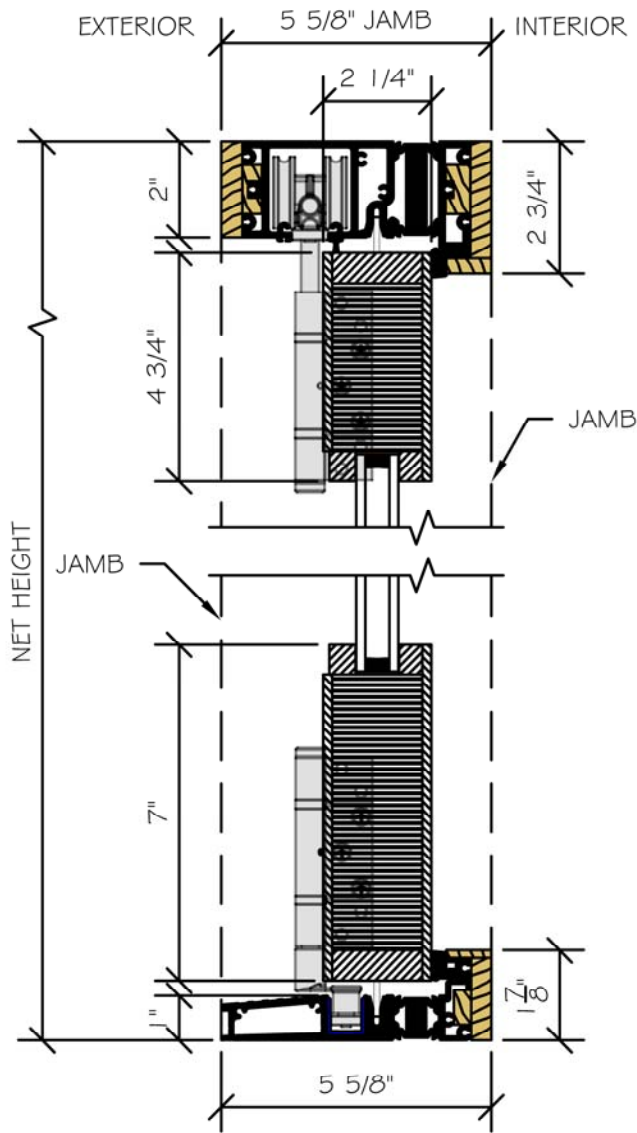
SECTION VIEW
