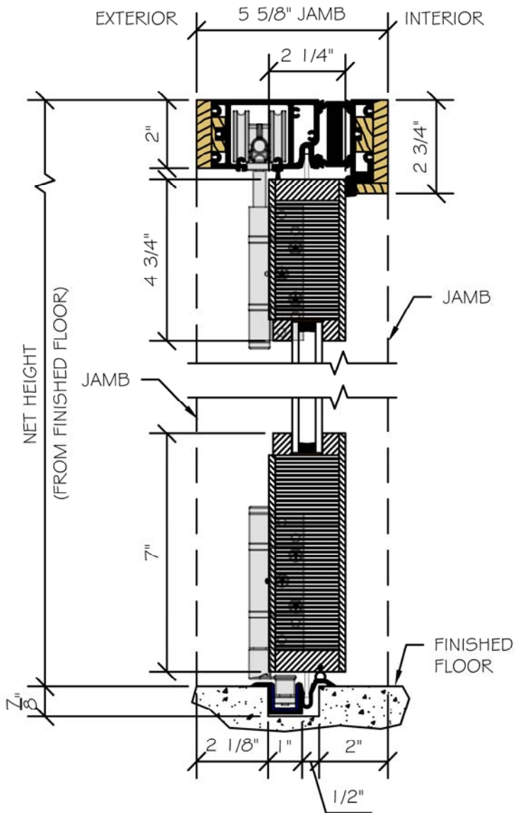
SECTION VIEW
