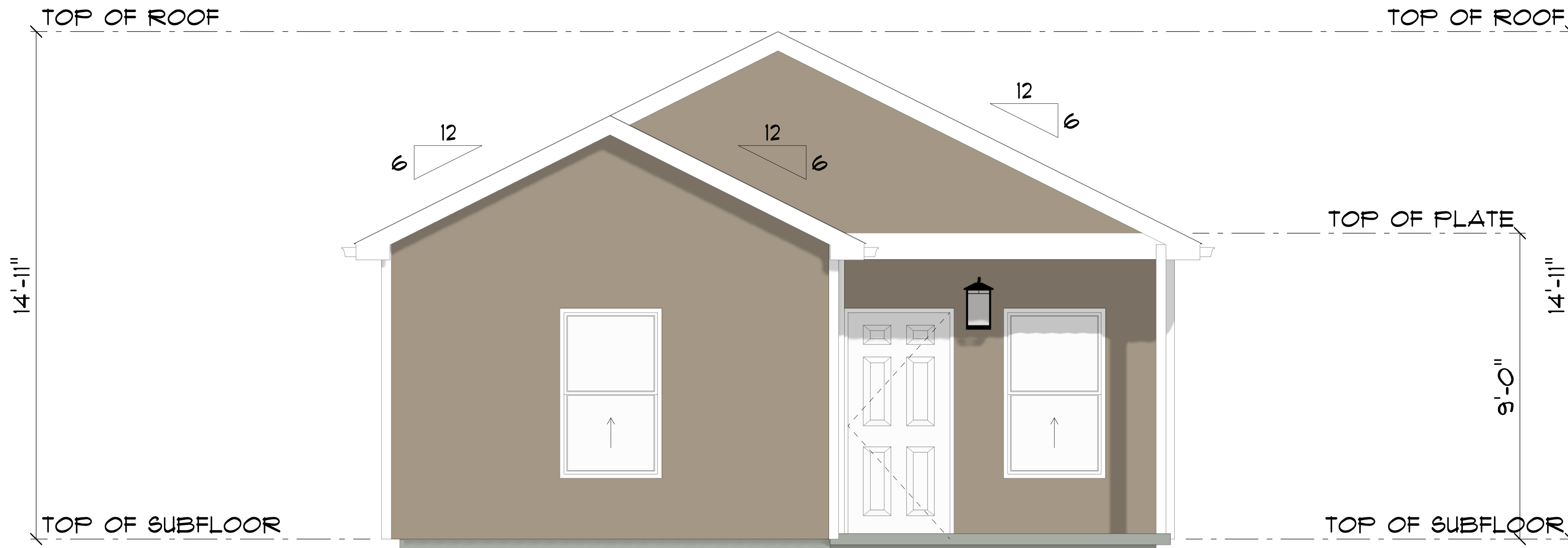
EAST ELEVATION SCALE: 1/2" = 1'-0"
